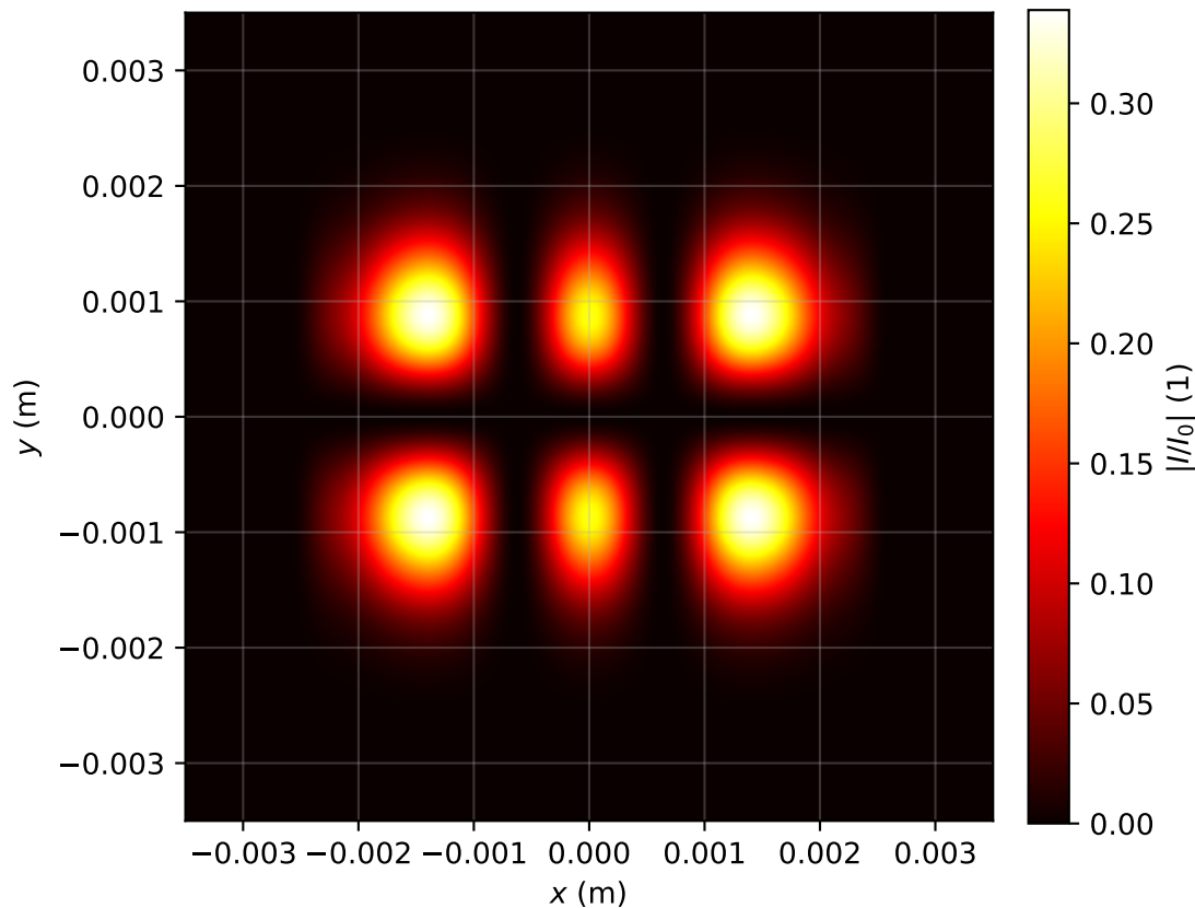
Intensity profile I(x, y, z = 2.946)/I_0 , P_{in}=0.5P_{cr} , artificial time
